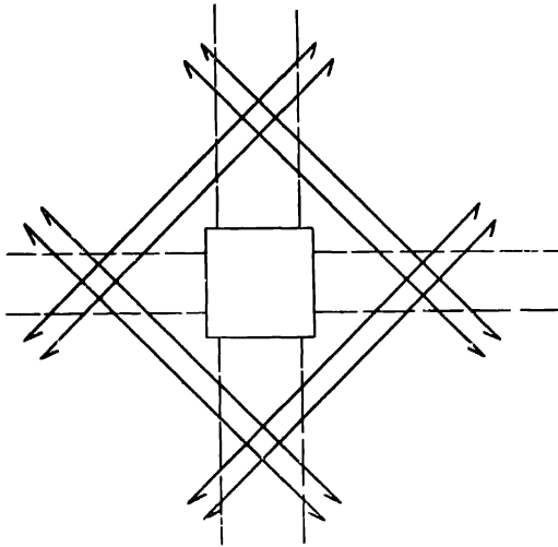
Fig. 250. Sketch showing Diagonal Bars around Column Head.
